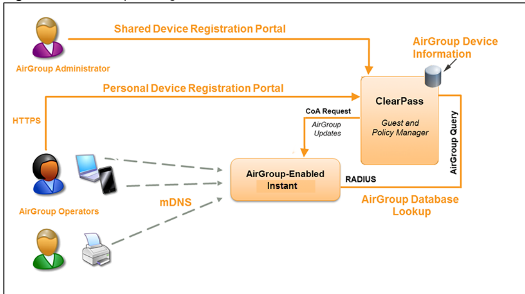
Figure 100 - AirGroup in a Higher-Education Environment
