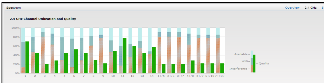
Figure 69 Channel Metrics for the 2.4 GHz Radio Channel
