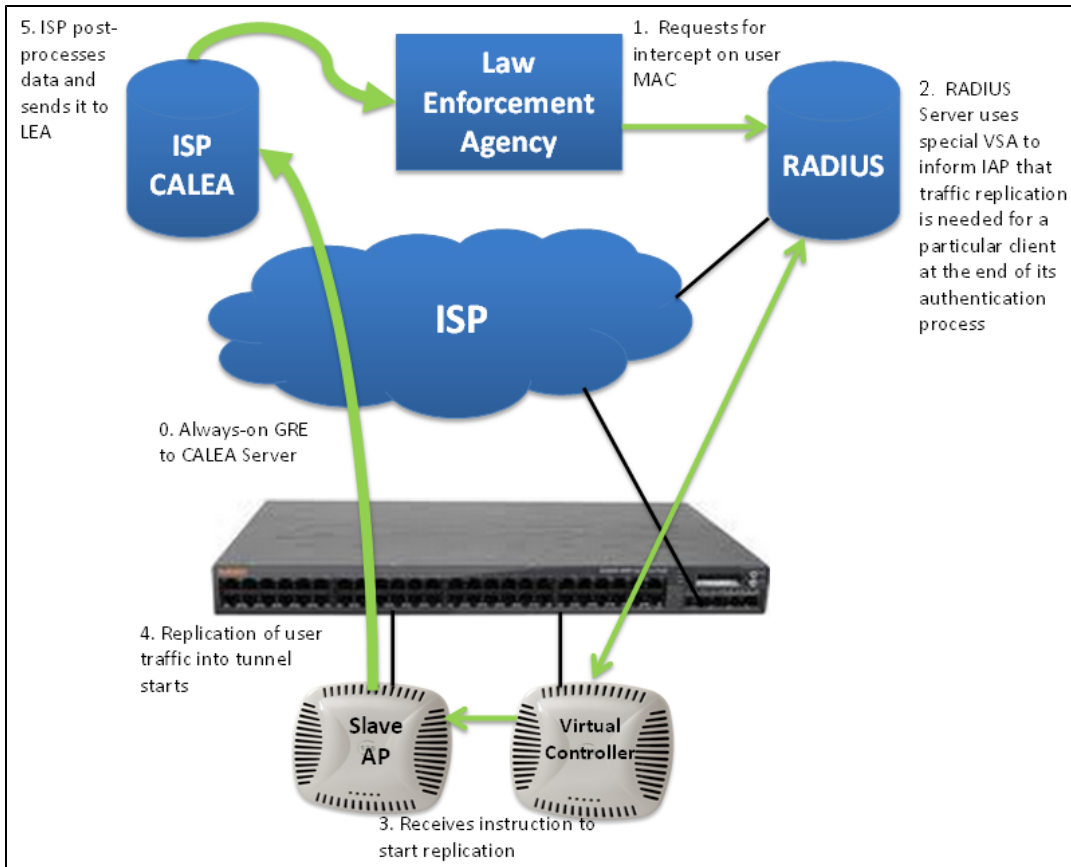
Figure 105 IAP to CALEA Server
