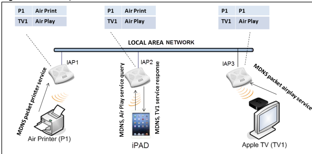
Figure 98 - AirGroup Architecture
