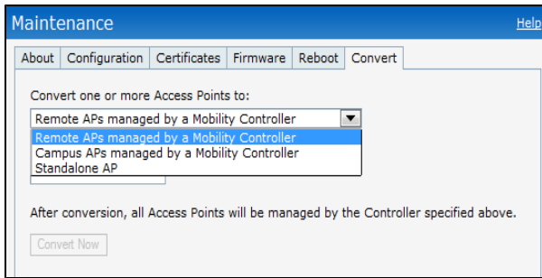
Figure 108 - Convert options
