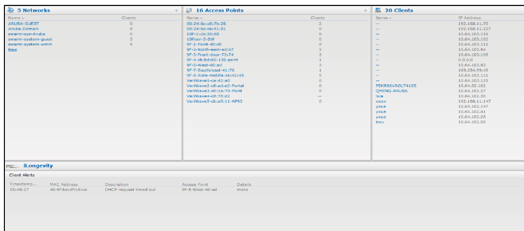
Figure 23 Client Alerts
