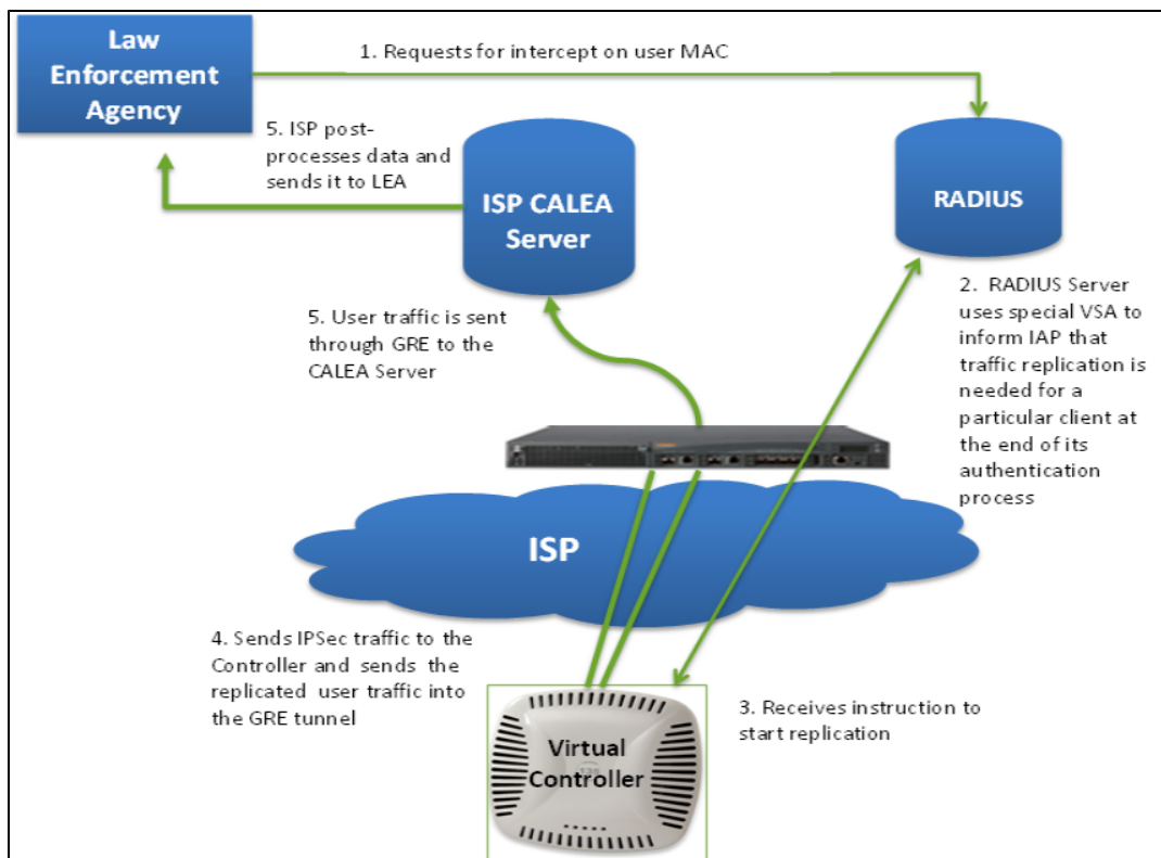
Figure 106 IAP to CALEA Server through VPN
