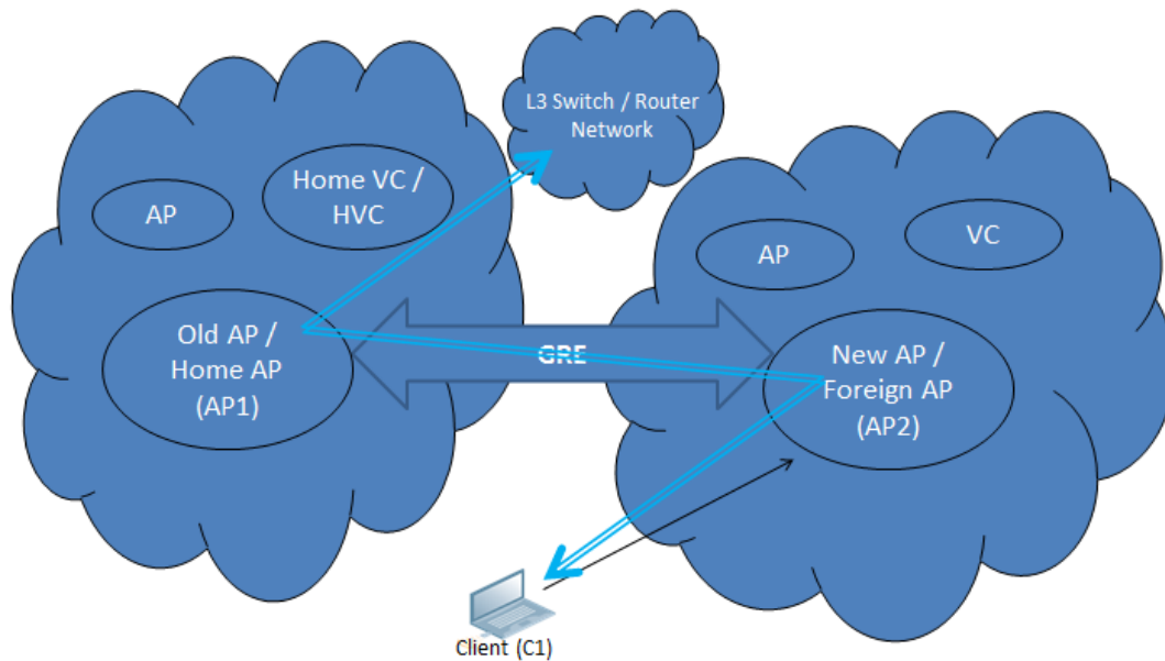
Figure 65 Routing of traffic when the client is away from its home network
