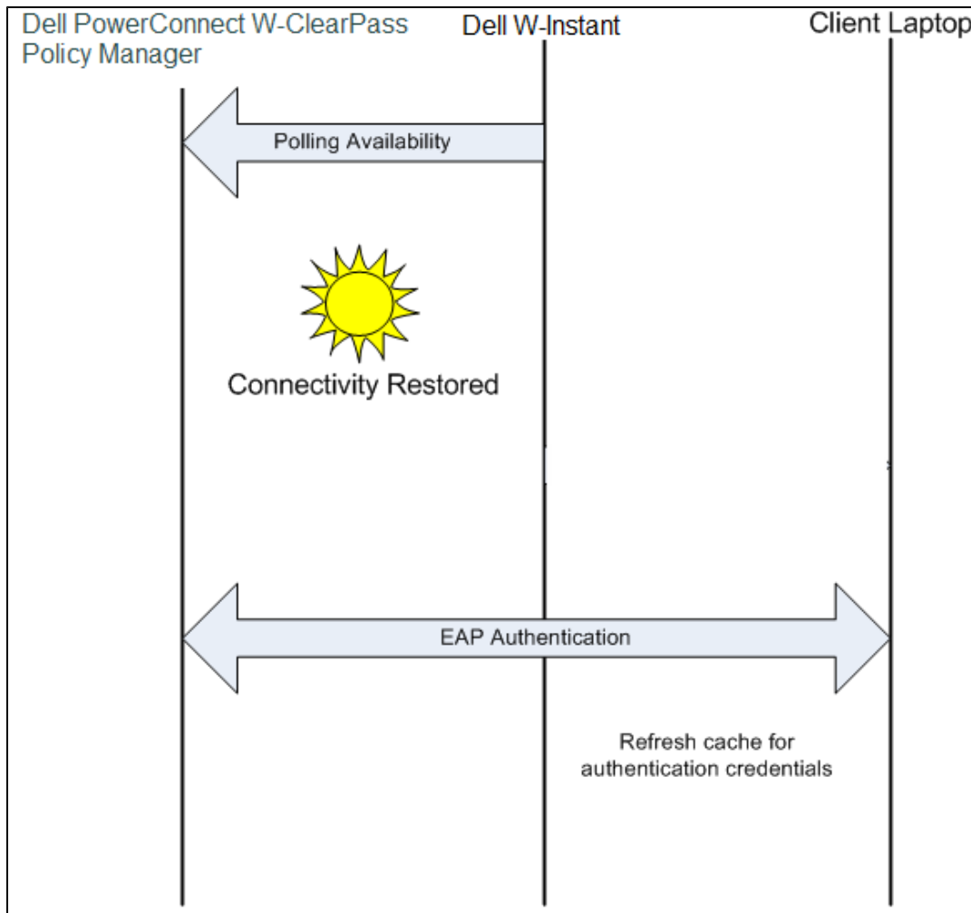
Figure 47 802.1X Authentication when CPPM is reachable again
