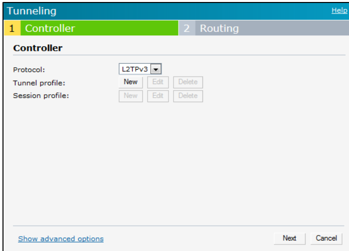
Figure 82 L3TPv3 Tunneling
