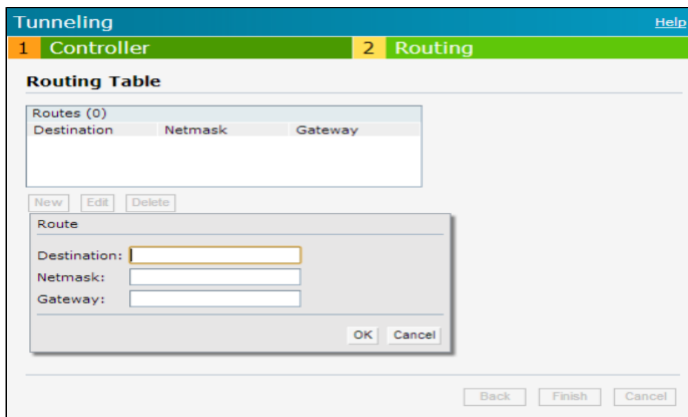
Figure 85 Tunneling— Routing
