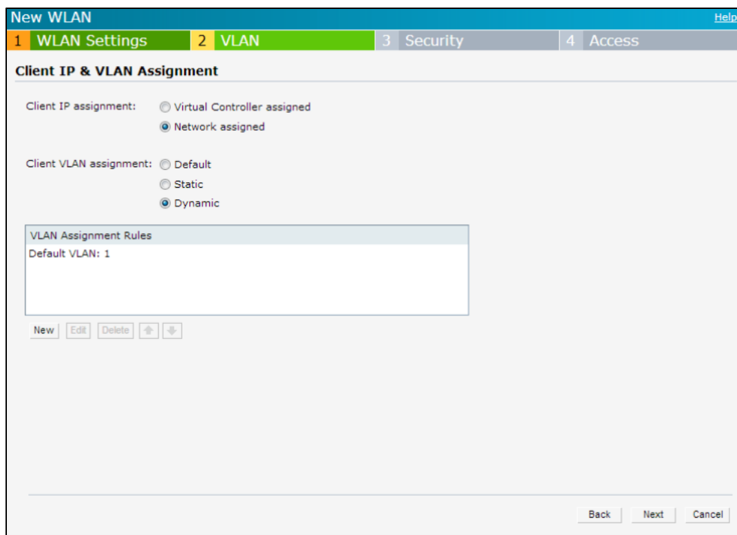
Figure 33 VLAN Tab
