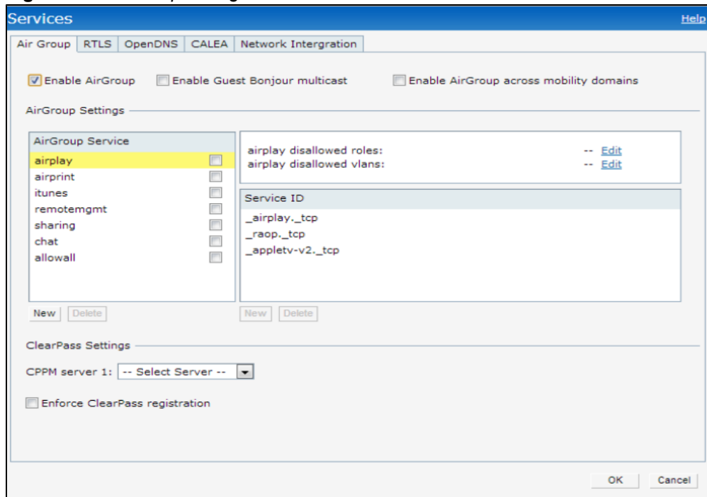
Figure 101 AirGroup Configuration
