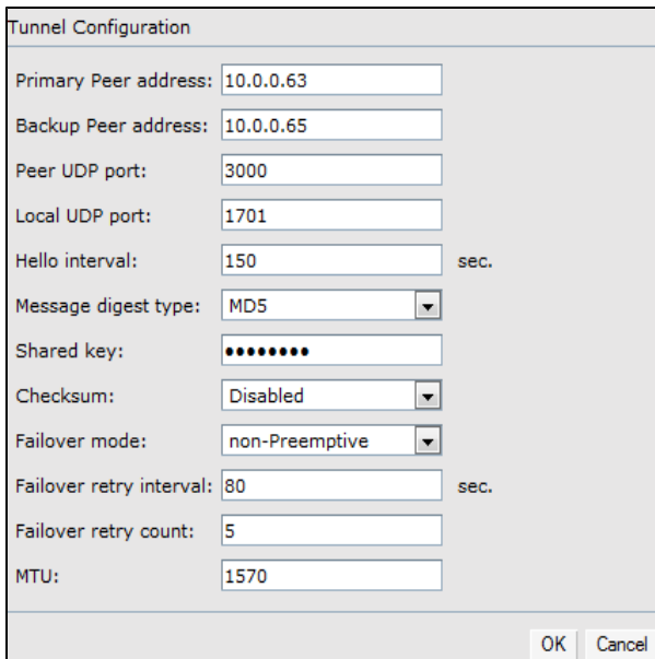
Figure 83 Tunnel Configuration
