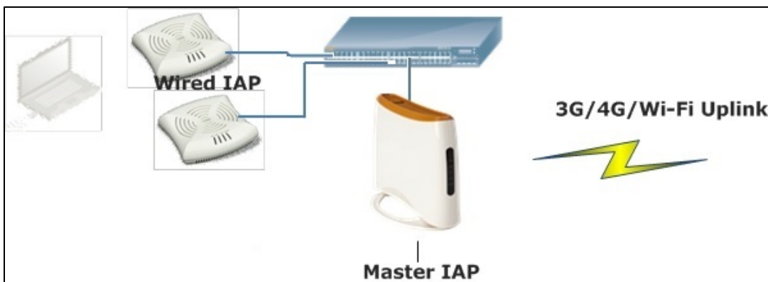
Figure 63 Uplink Types
