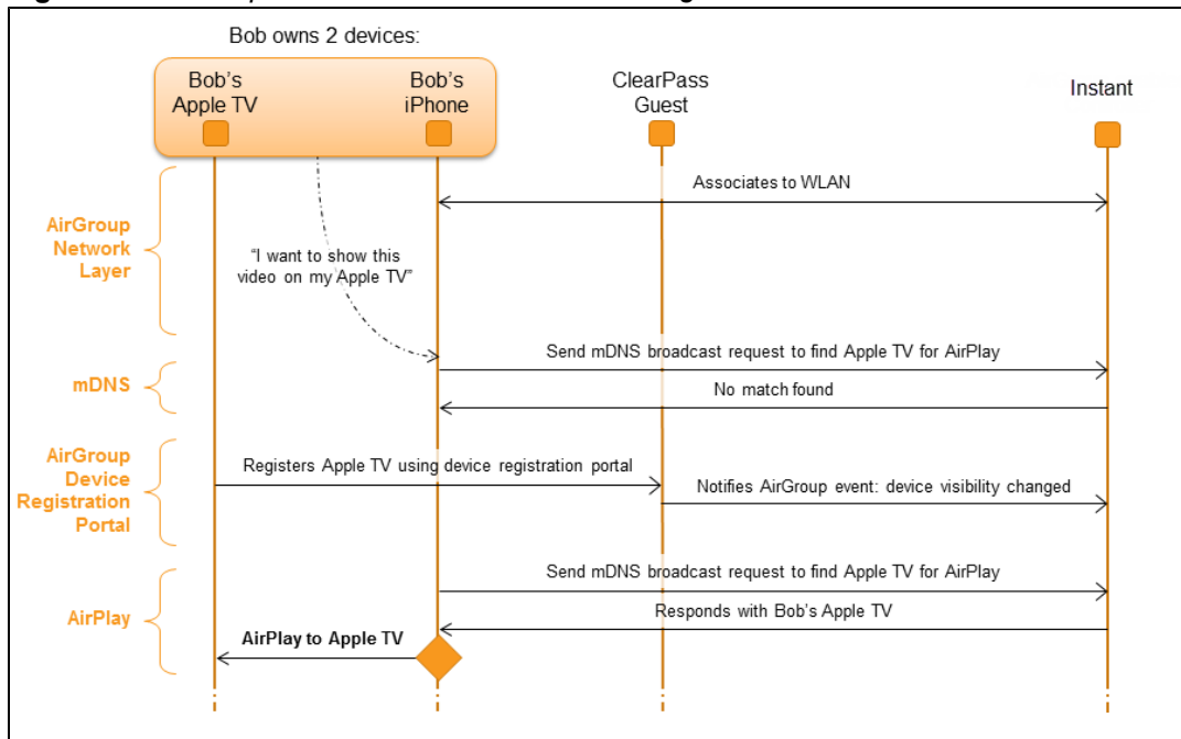
Figure 99 AirGroup Enables Personal Device Sharing
